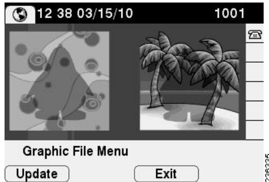
Figure 3-13 CiscoIPPhoneGraphicFileMenu
