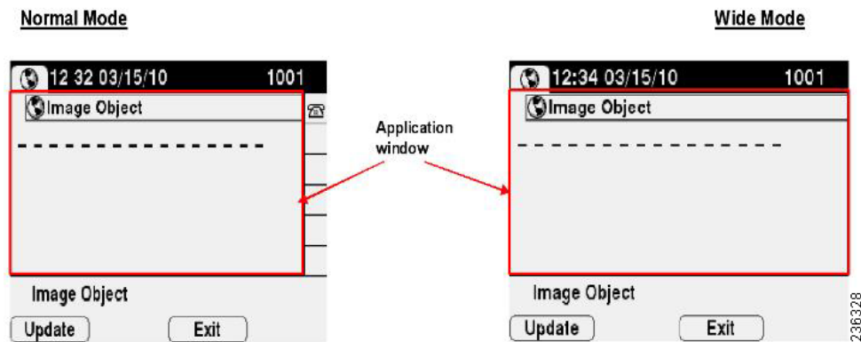
Figure 3-3 WindowMode
