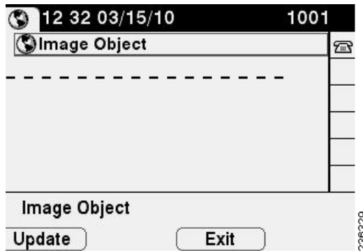
Figure 3-5 CiscoIPPhoneImage Object
