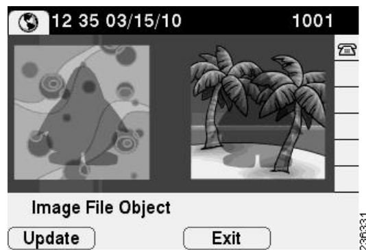
Figure 3-8 CiscoIPPhoneImageFile Object
