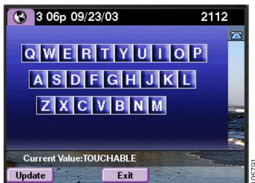
Figure 3-12 CiscoIPPhoneGraphicFileMenu
