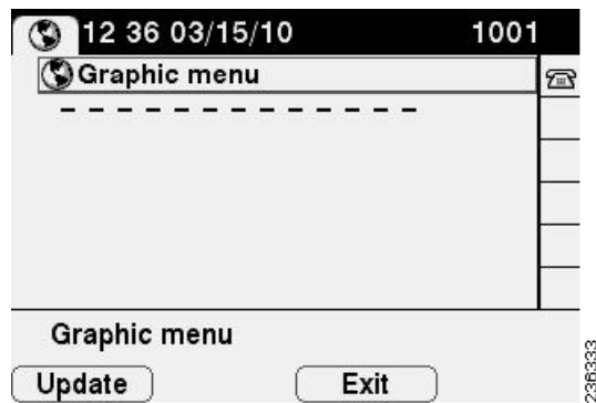
Figure 3-10 CiscoIPPhoneGraphicMenu Object
